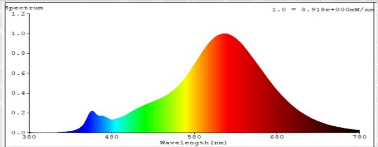
Model: 97260 (2200K)
